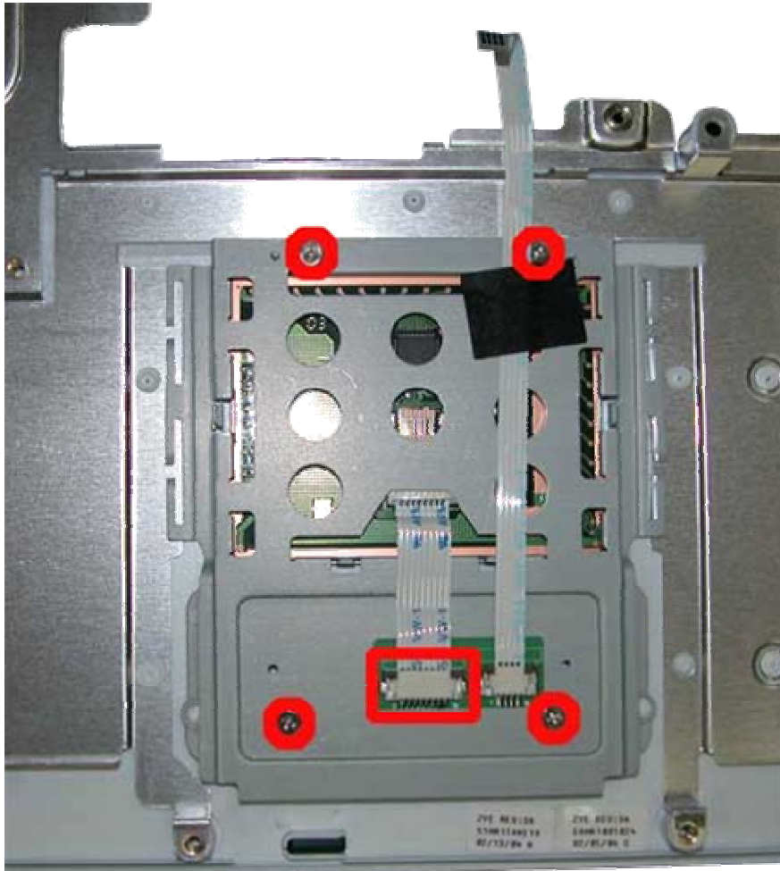
Fig. 27 Touch Pad
